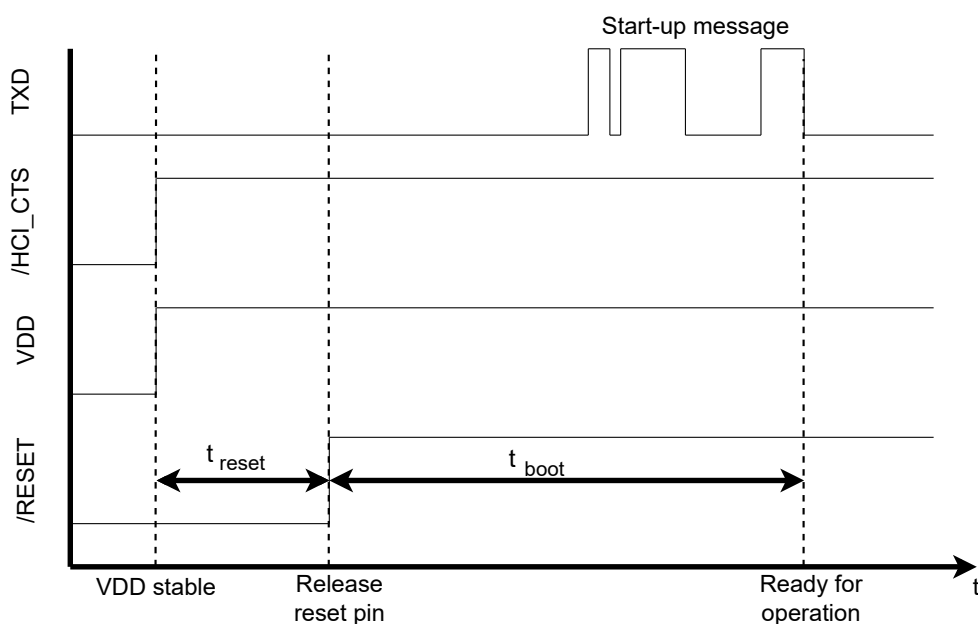
Figure 5: Power up
